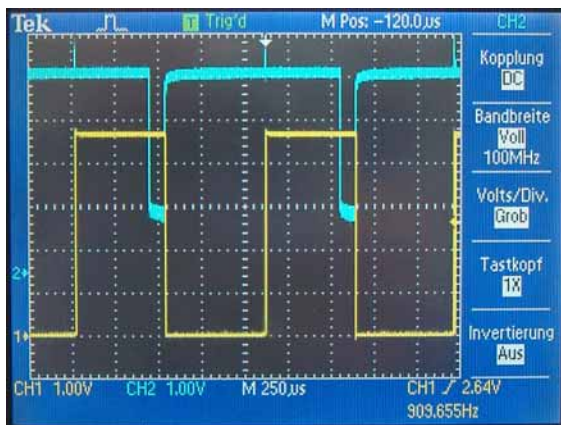
capture mode 3 (910Hz, sh = 1000 \mu\text{s} , TRIGINP_NEG(), TRIGOUT_POS())
