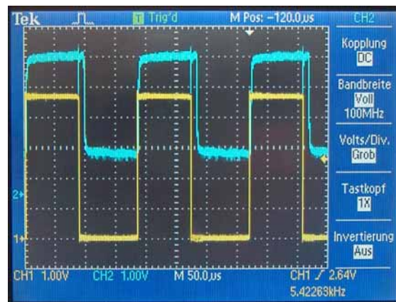
capture mode 3 (5,422kHz, sh = 90 \mu\text{s} , TRIGINP_POS(), TRIGOUT_POS())
